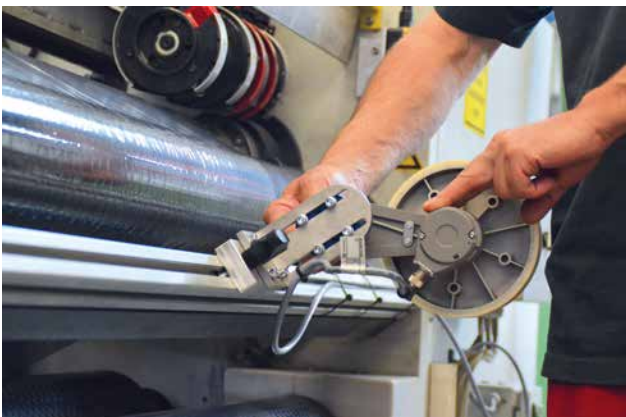
WA1701_3 Since the wheel measures the metres of film, it measures directly on the film itself. When changing the rolls or performing other work on the conveyor belt, the spring arm can be folded away and locked in a few simple steps.
